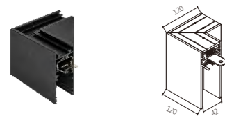
Sideward 90°connector (to be ordered separately)
