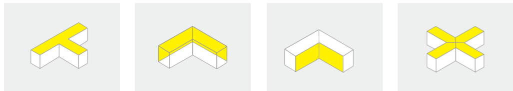
"T" shape connector T90 Outward 90° connector Inward 90° connector Cross shape connector X90
