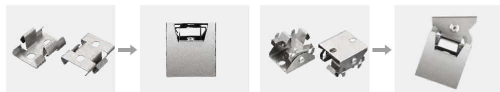
Fixed mounting clips After installation Adjustable mounting clips After installation
