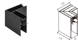
Sideward 90°connector (to be ordered separately)
