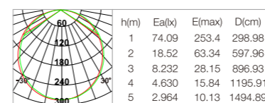
Beam Angle 110° 16W 4000K
