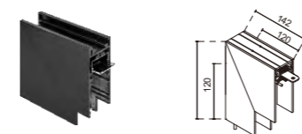
Inward 90°connector (to be ordered separately)
