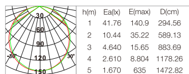
Beam Angle 110° 8W 4000K
