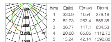
Beam Angle 110° 64W 4000K
