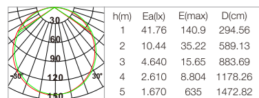
Beam Angle 110° 8W 4000K
