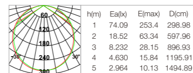
Beam Angle 110° 16W 4000K
