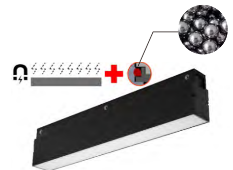
Ball catch design, more safe
